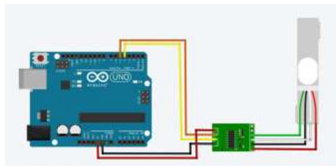
Figure 3: Fuel weight scale schematic diagram
