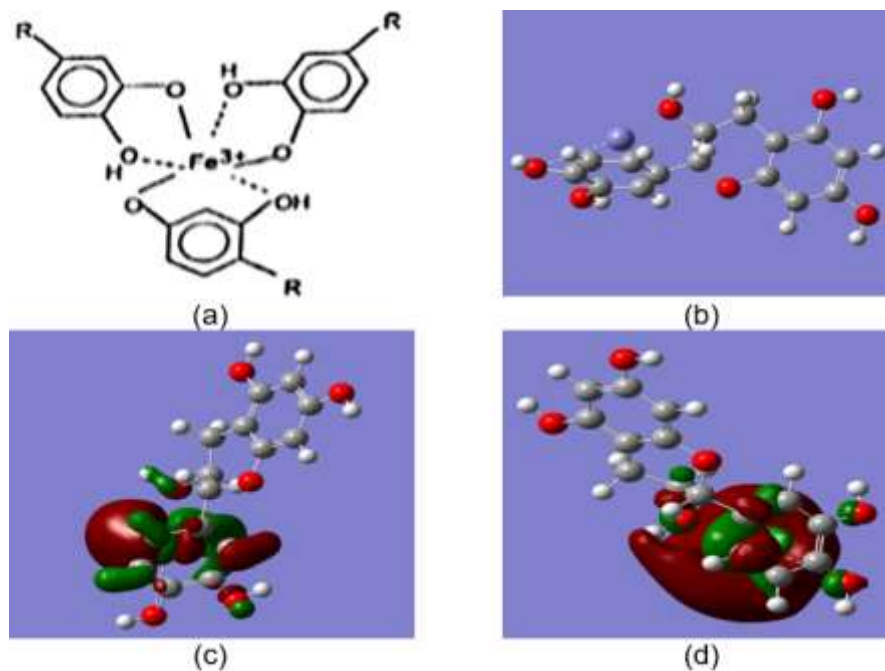
Figure 6: Optimization process for tannin-Fe compounds, (a) Molecular structure (b) Geometry structure (c) HOMO Contour, and (d) LUMO Contour
