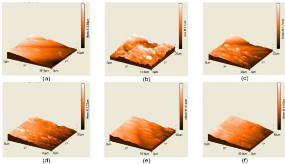
Figure 4: Morphological of steel surfaces using an AFM (a) without Treatment, (b-f) Treatment in variations in immersion time in inhibitors. (b) without inhibitors (c) 24 hours (d) 72 hours (e) 120 hours (f) 168 hours with 1.5M HCl medium
