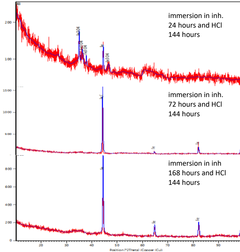
Figure 3. XRD characterisation results for samples at variation time (hour) of inhibitor in the corrosive medium HCl 1.5M for 144 hours (a) 24, (b) 72, and (c) 168.
