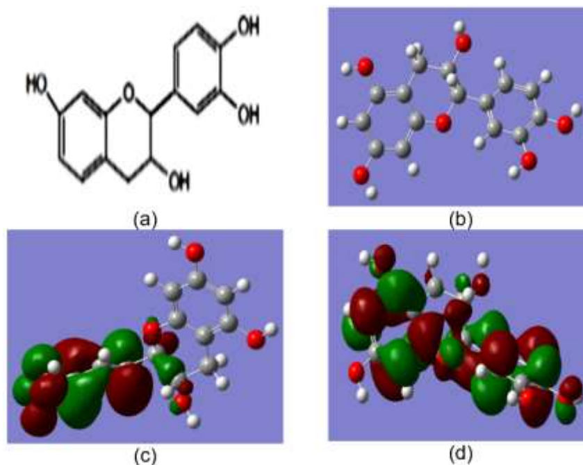
Figure 5: Process of tannin compound optimisation, (a) Structure of molecular (b) Structure of geometry, (c) Contour of HOMO, and (d) Contour LUMO
