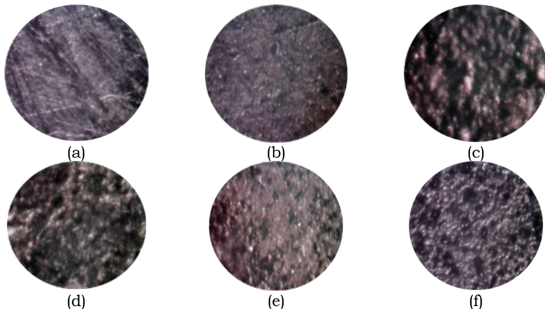
Figure 1: Steel surface morphology using an optical microscope in 1.5 M HCL medium for 144 hours with variations in immersion time in inhibitors with 100X magnification (a) without treatment (b) without inhibitors (c) 24 hours (d) 72 hours (e) 120 hours and (f) 168 hours
