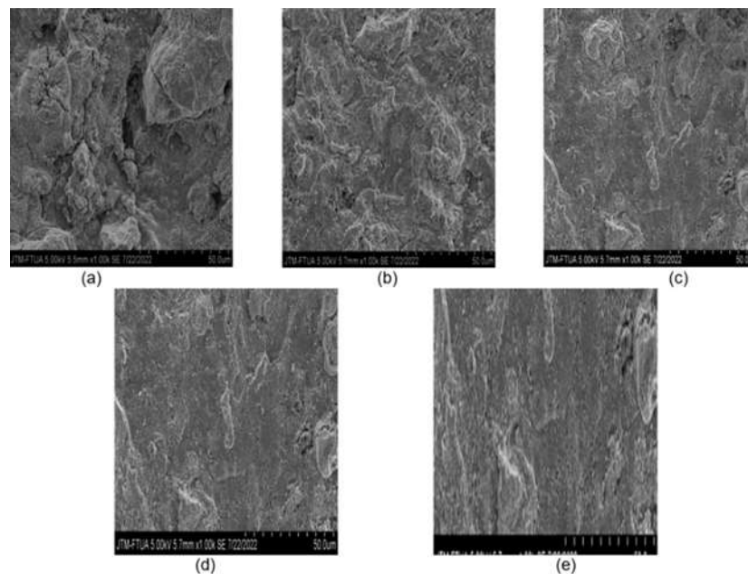
Figure 2: Morphology of steel surfaces by SEM in 1.5 M HCl medium for 144 hours with variations in immersion time in inhibitors with 1000X magnification (a) without Inhibitors, (b) 24 hours, (c) 72 hours, (d) 120 hours, and (e) 168 hours
