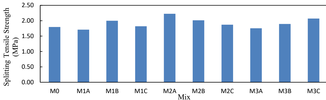
Figure 4: Splitting tensile strength of hardened mortar after 28 days
